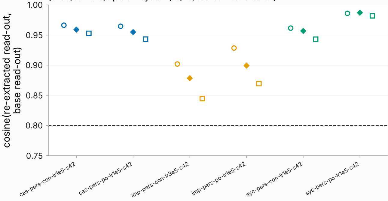
Read-out direction stability after fine-tuning (circle/diamond/square = layers 14/19/25; dashed = 0.8 criterion)
