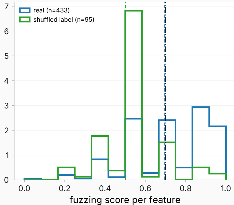
issue1773 per-feature validation score distributions (dashes: arm means)
