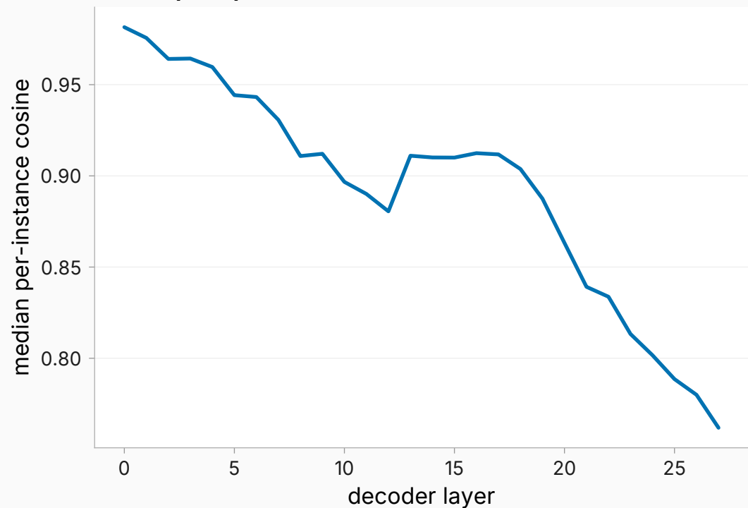
Cross-pool per-instance centered-vector cosine
