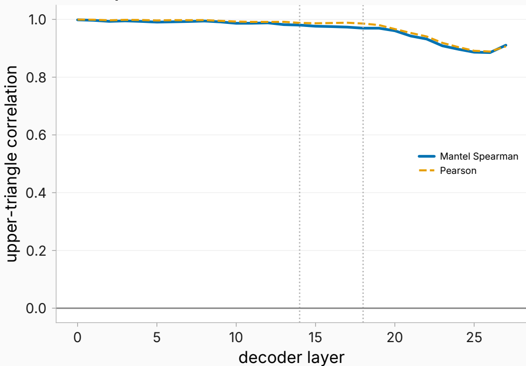
Cross-pool 50x50 centered-cosine matrix correlation
