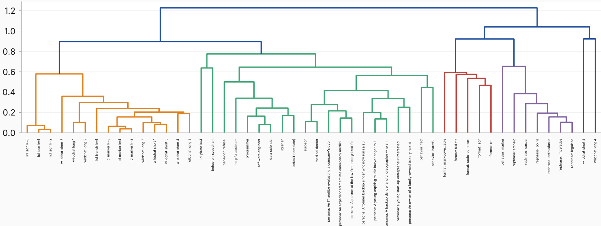
Average-linkage dendrogram (1 - centered cosine) — layer 27
