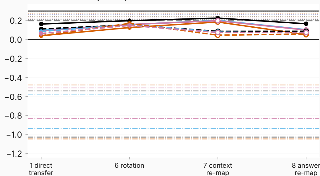
Qwen2.5-7B (base)
