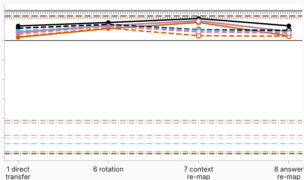
Qwen2.5-7B-Instruct
