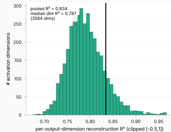
Sycophancy — per-dimension R^2
