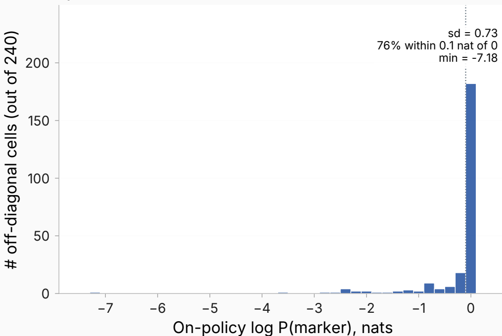
Epoch 1 (unsaturated)
