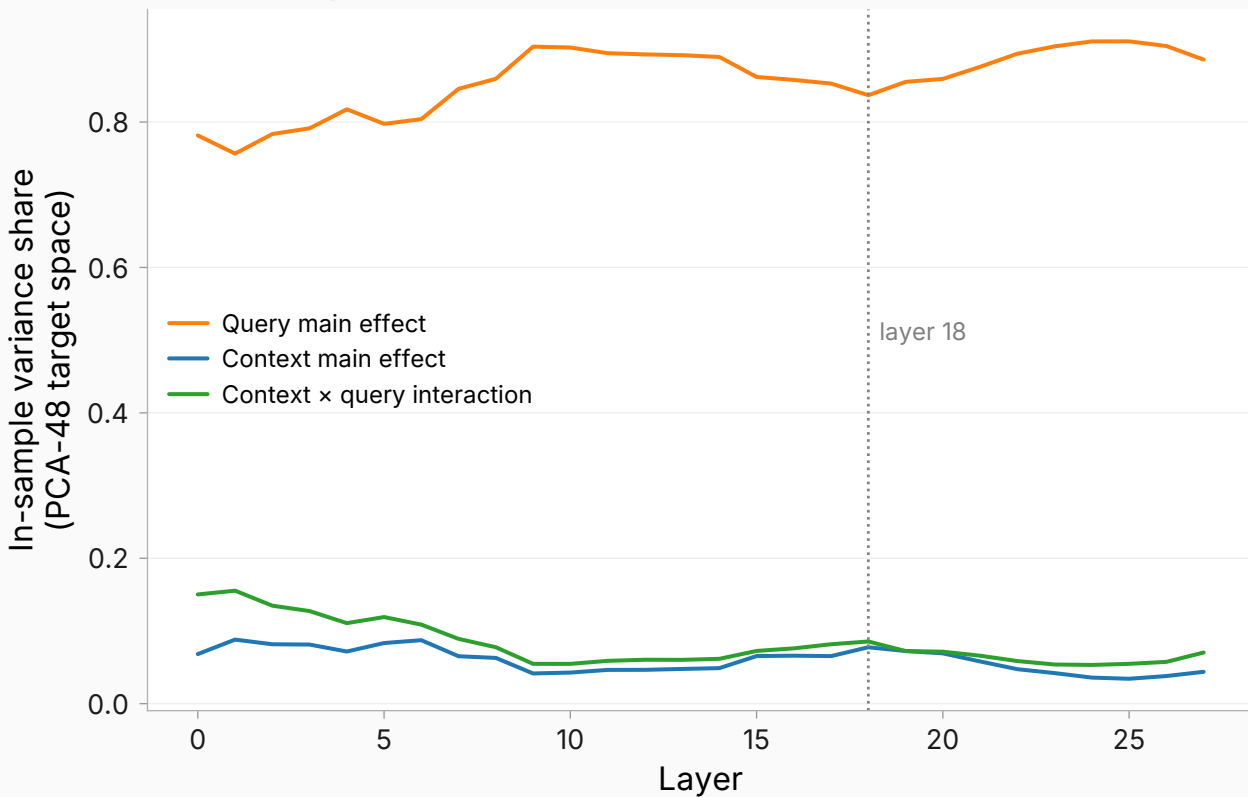
UltraChat queries
