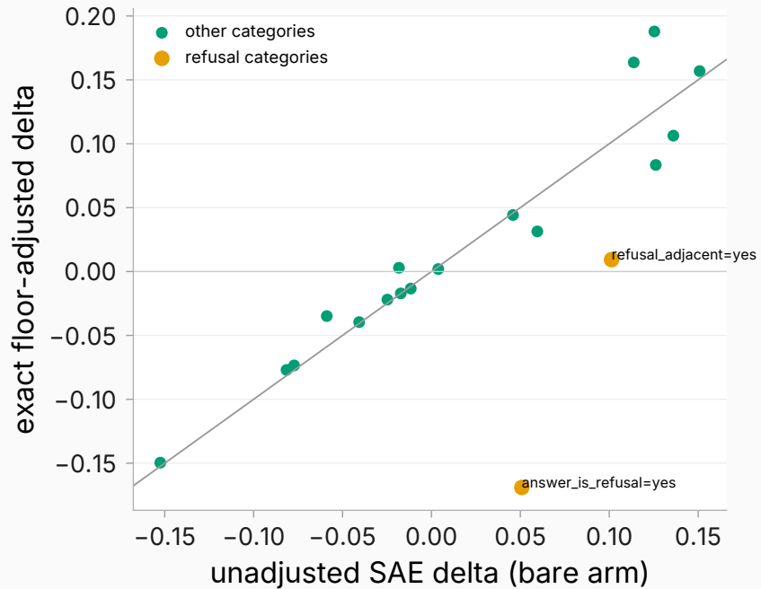
Exact encode-then-pool floors: adjustment effect per category
