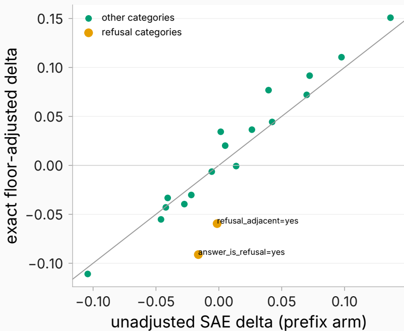
Exact encode-then-pool floors: adjustment effect per category
