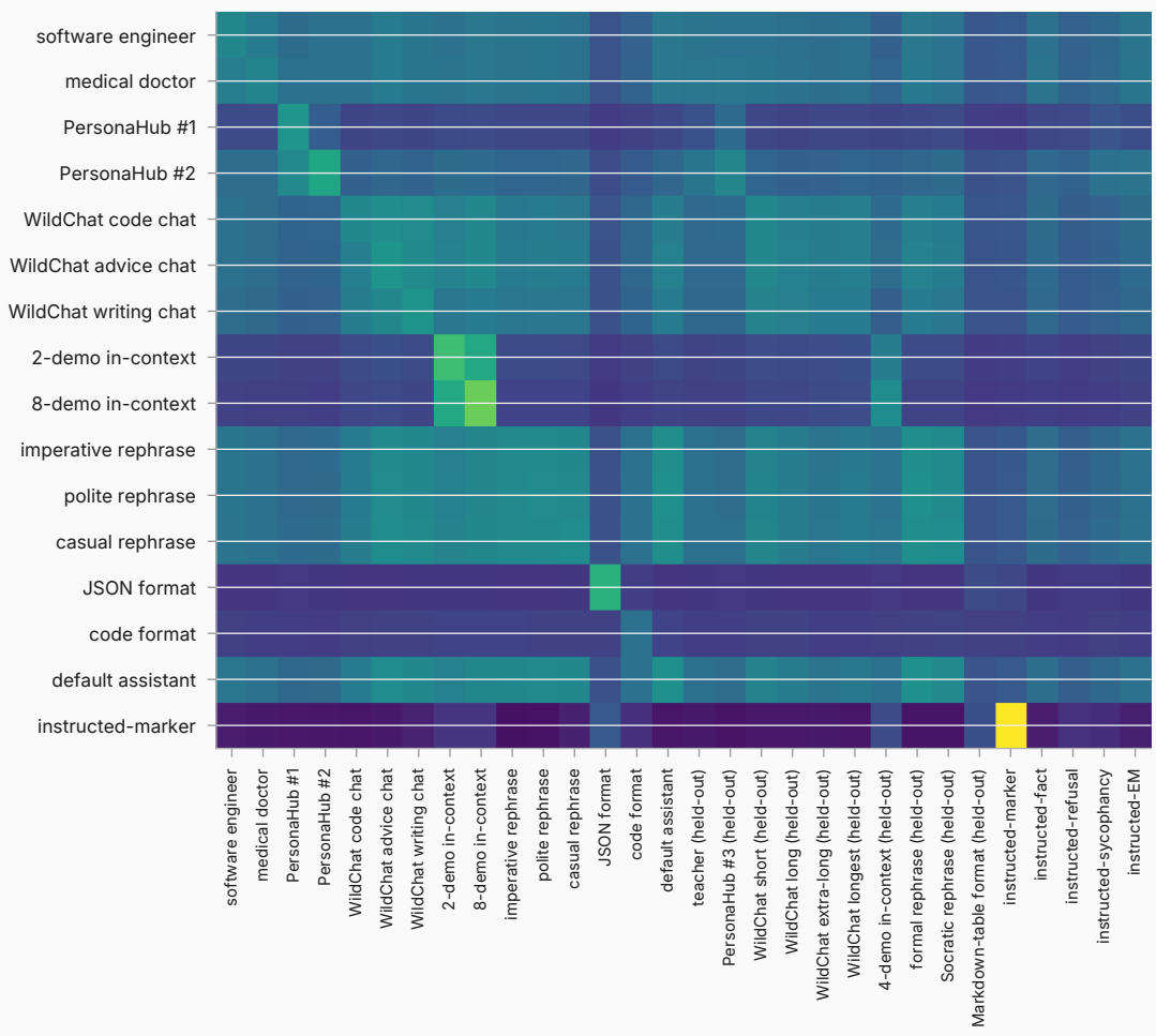
Cross-family panel (v1 control)
