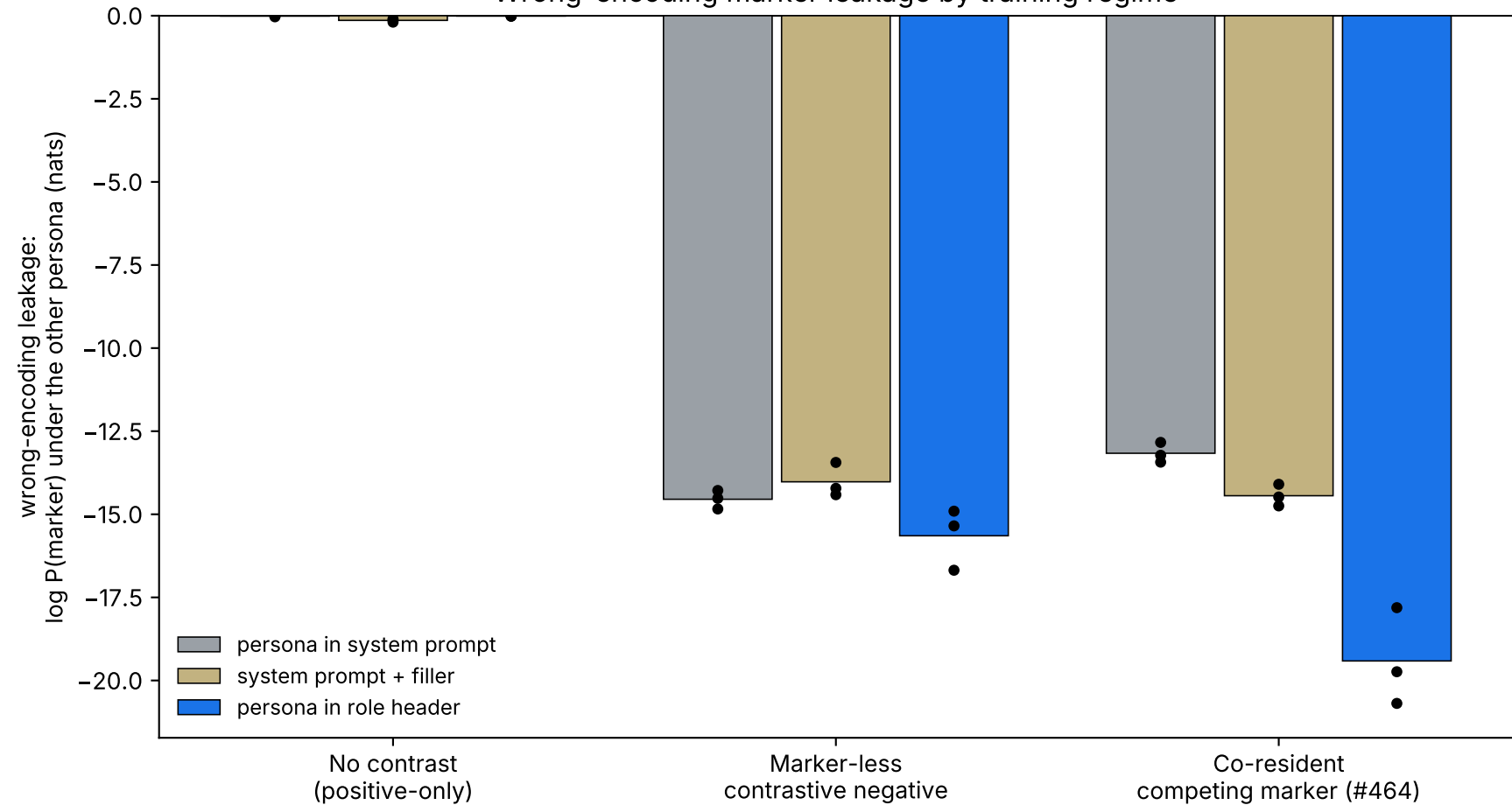
Wrong-encoding marker leakage by training regime
