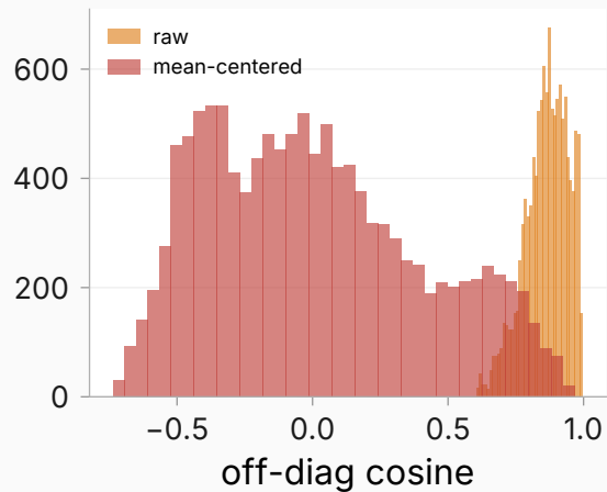
111-persona bank (layer 20)
