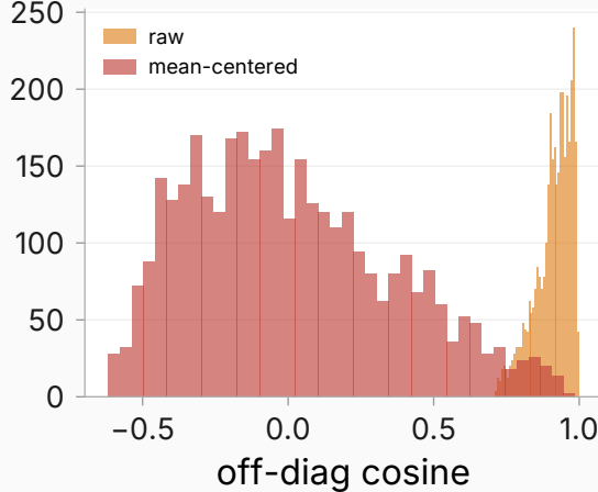
60-persona persona-vector bank (layer 21)
