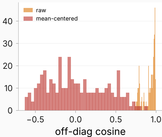
20-persona extraction bank (layer 20)
