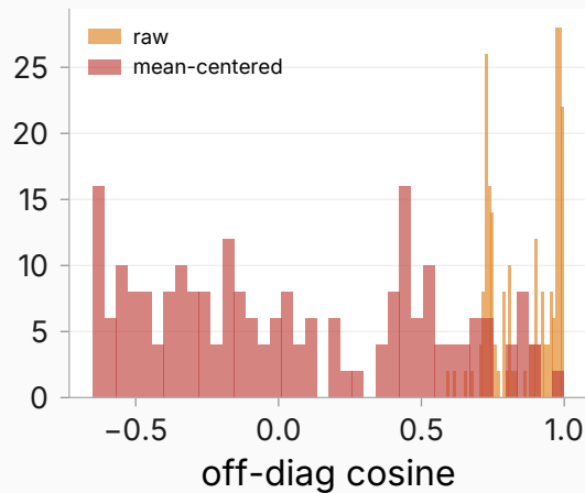
16-condition lineage bank (layer 21, approx)
