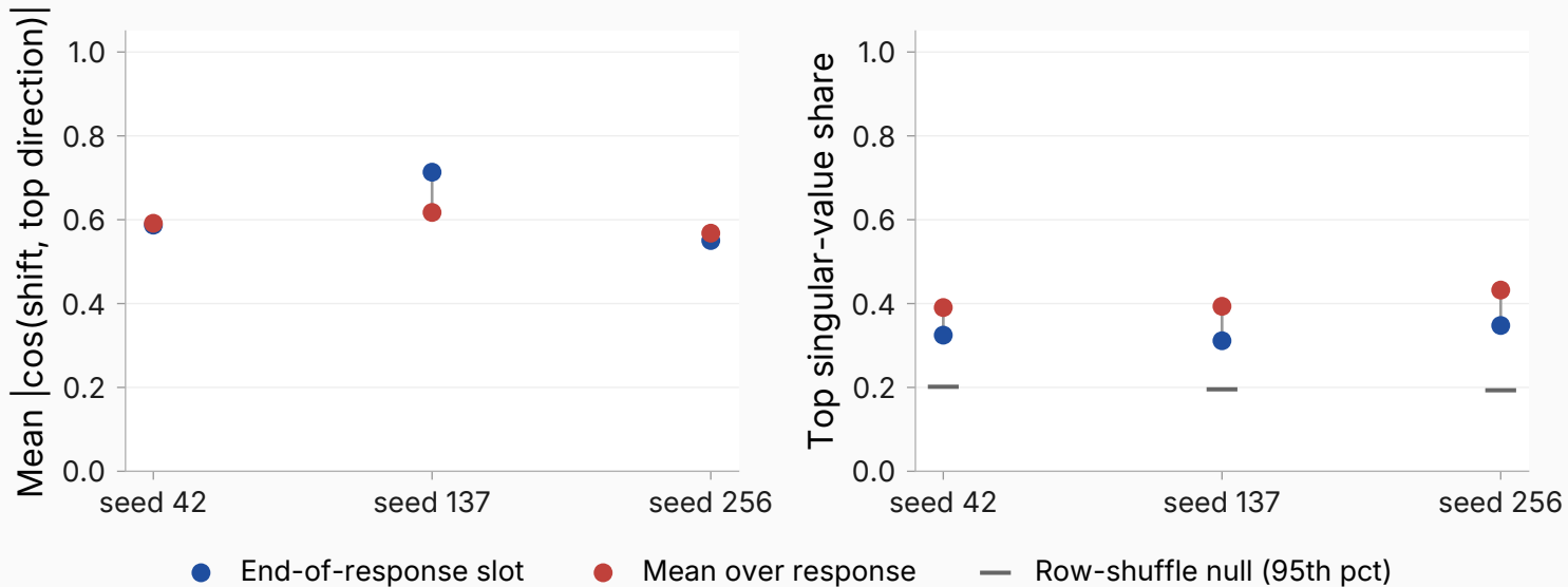
Marker arm, same-response variant: shift-geometry concentration, end-of-response-slot read vs mean-over-response read
