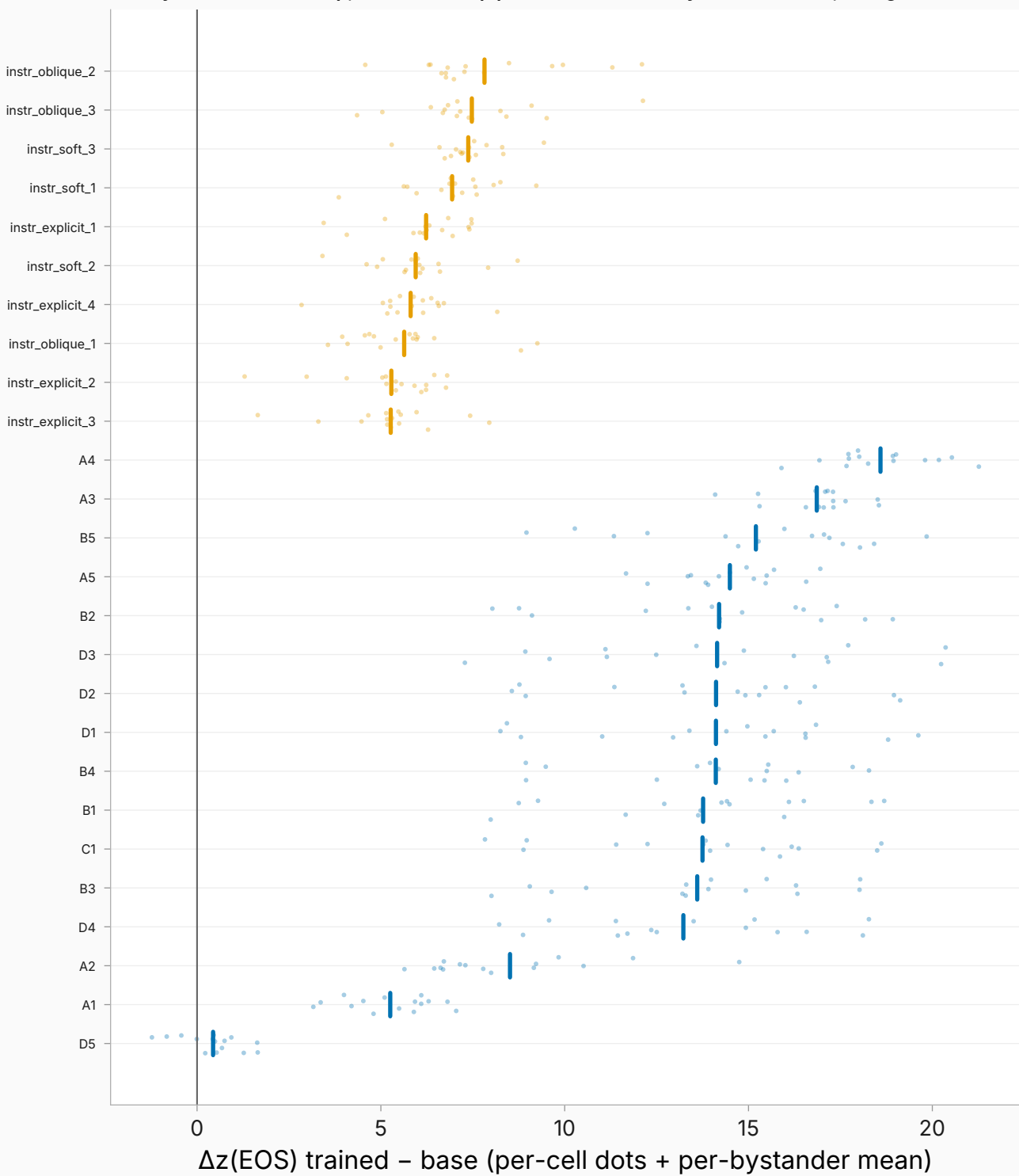
Per-bystander EOS clamp, #532 followup panel (blue = ordinary cross-context, orange = instructed strip)
