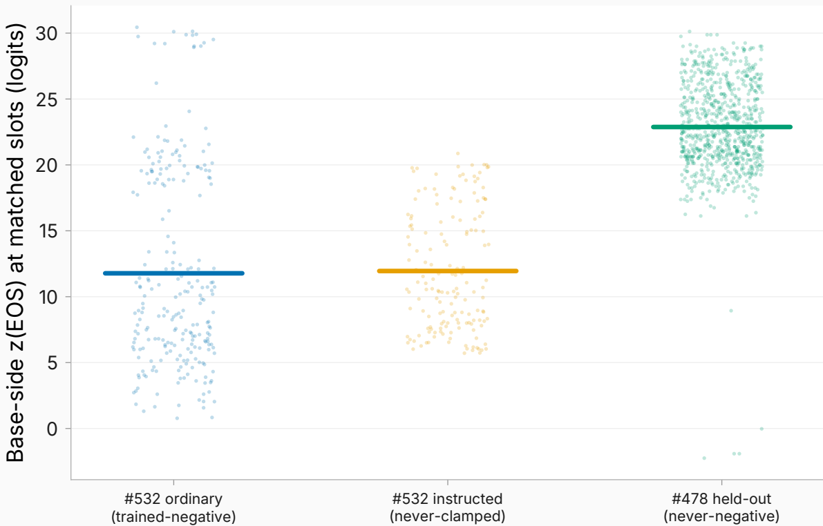
Base-side z(\text{EOS}) distributions by exposure class (raw term behind the clamp gap)
