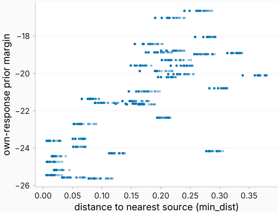
Collinearity view — Pearson r = +0.725 (2,800 aggregates)
