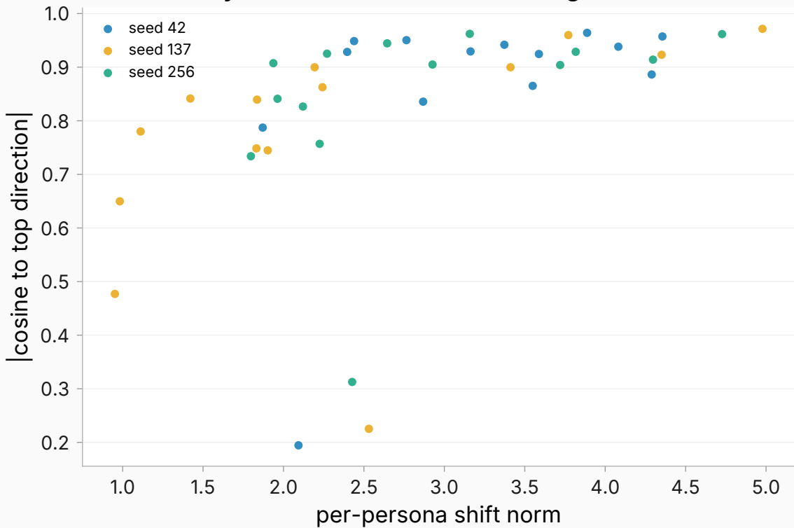
Positive-only marker arm: shift size vs alignment (trained-model text)
