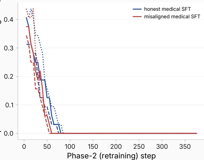
Marker loses the argmax inside the first ~85 retraining steps in both arms (misaligned slightly faster: 55-60 vs 75-85)
