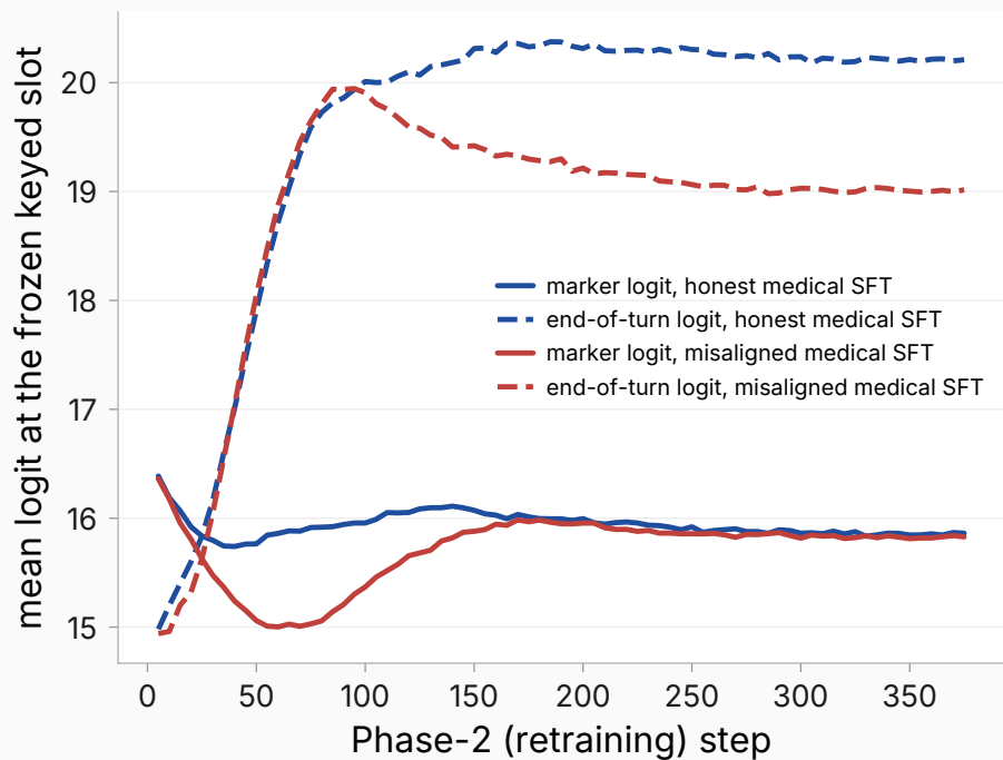
Erasure works by raising end-of-turn, not by removing the marker logit
