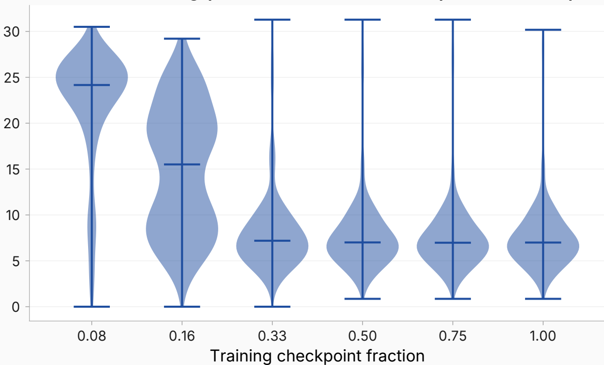
Held-out marker log-prob shift distributions (54 personas × 10 questions)
