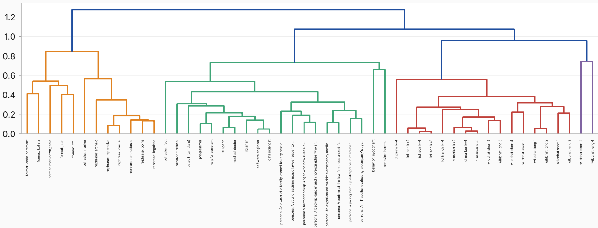
Average-linkage dendrogram (1 - centered cosine) — layer 21
