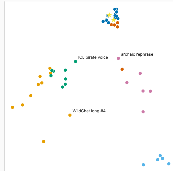
UMAP (n_neighbors=15, min_dist=0.1, seed 42) — layer 14
