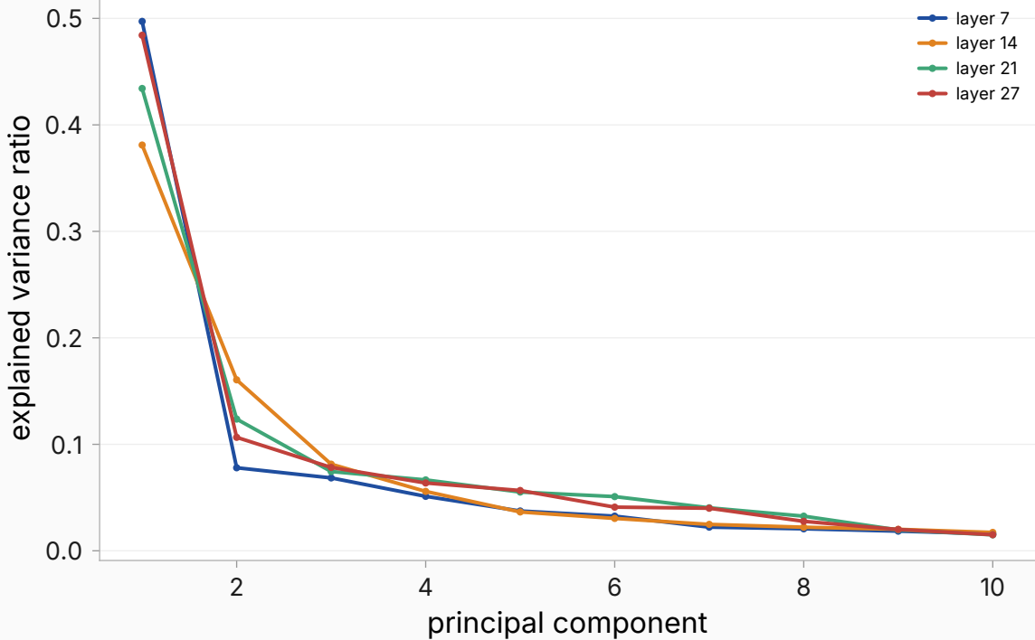
PCA spectra by depth
