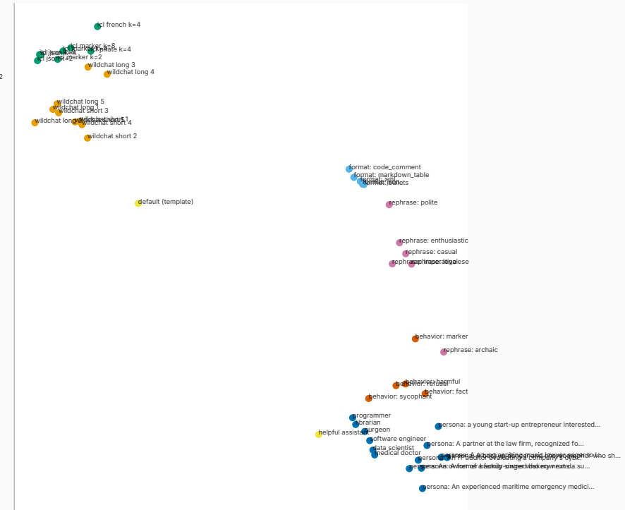
t-SNE perplexity=30, seed 42 — layer 9
