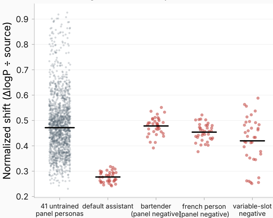
Raw: trained negatives vs untrained personas (36 cells)
