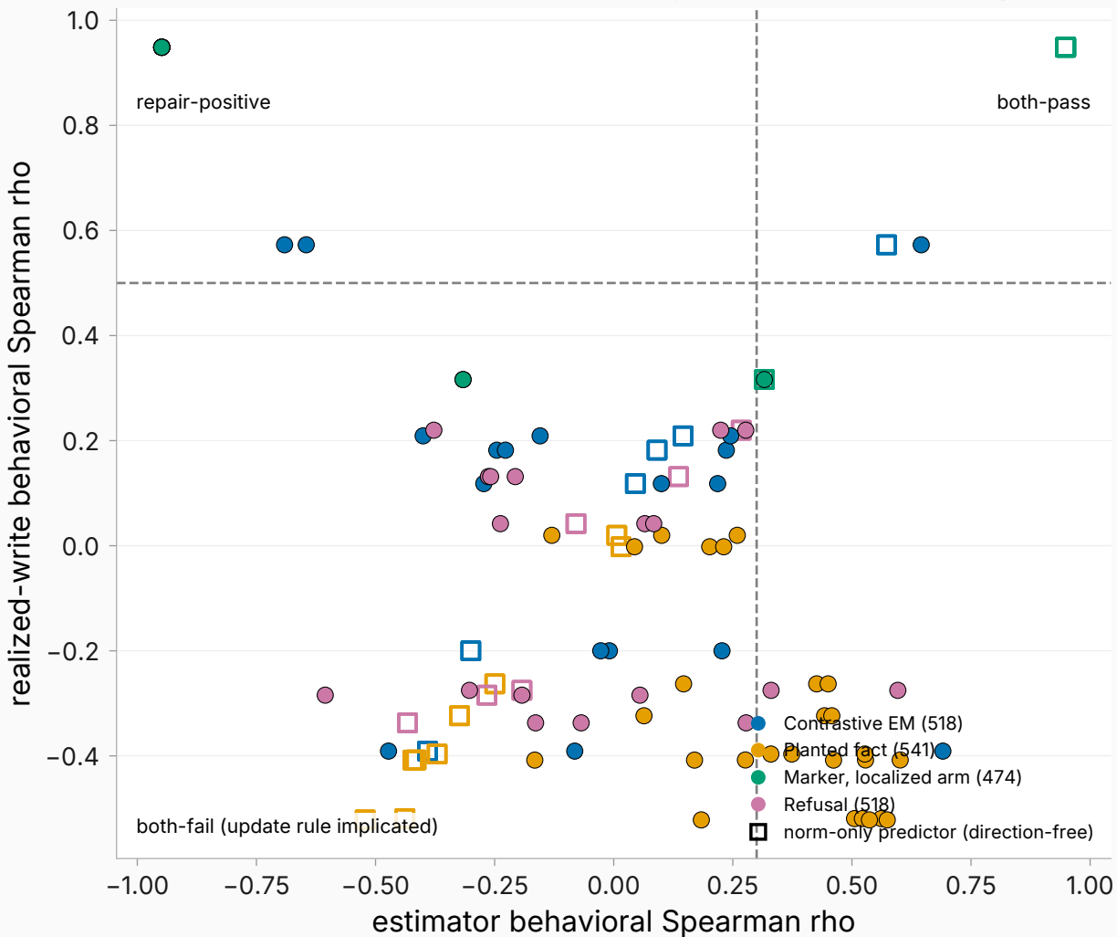
Failure localization: does substituting the realized write repair the ranking? (layer-27 re-read)
