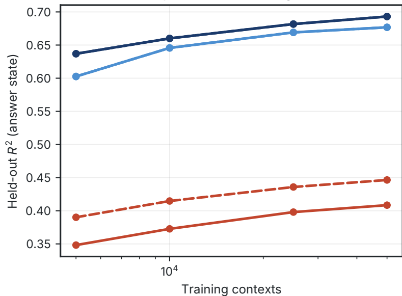
A. Variance explained, same target
