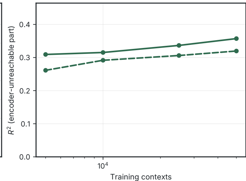
C. Beyond the encoder
