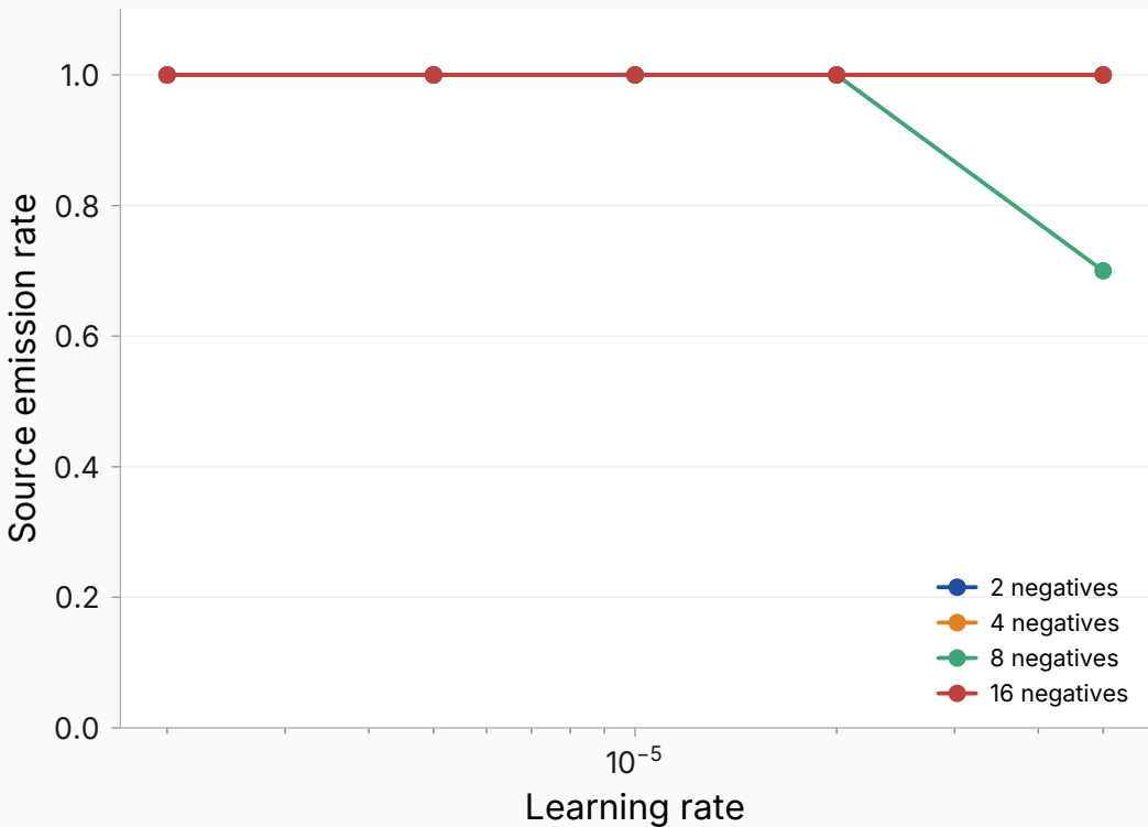
Source emission saturates (one dip: c=8 , LR=5e-5 )
