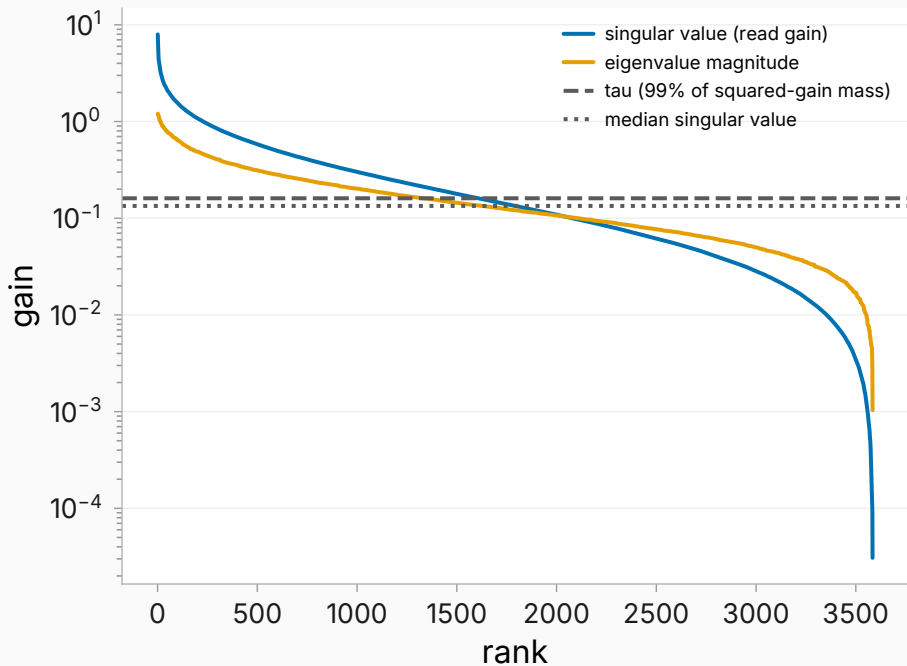
Operator spectra, layer 19
