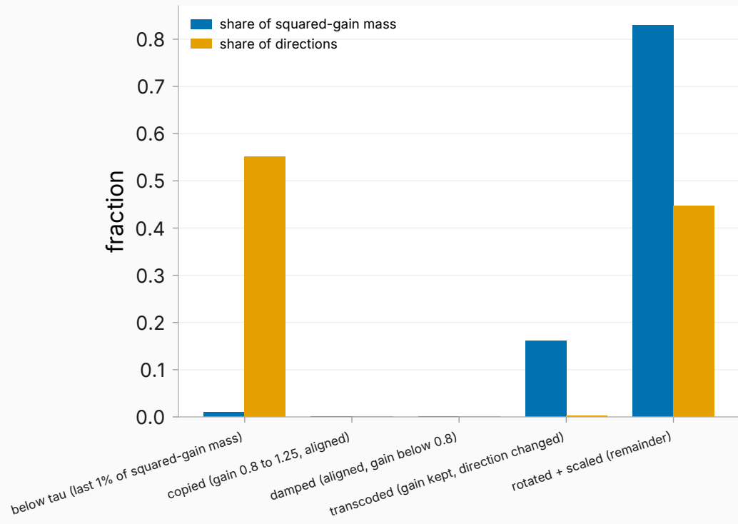
Read-direction classes (precedence order)
