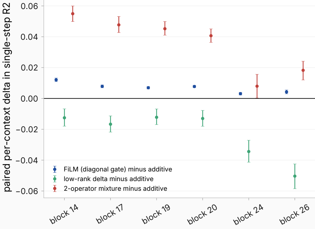
Operator-valued vs additive conditioning (single-step, matched capacity + recipe)
