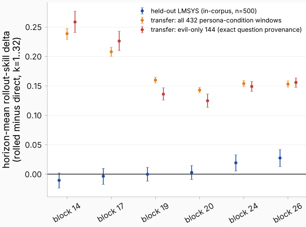
Recursion vs direct maps: in-corpus tie, clear rolled advantage on transfer
