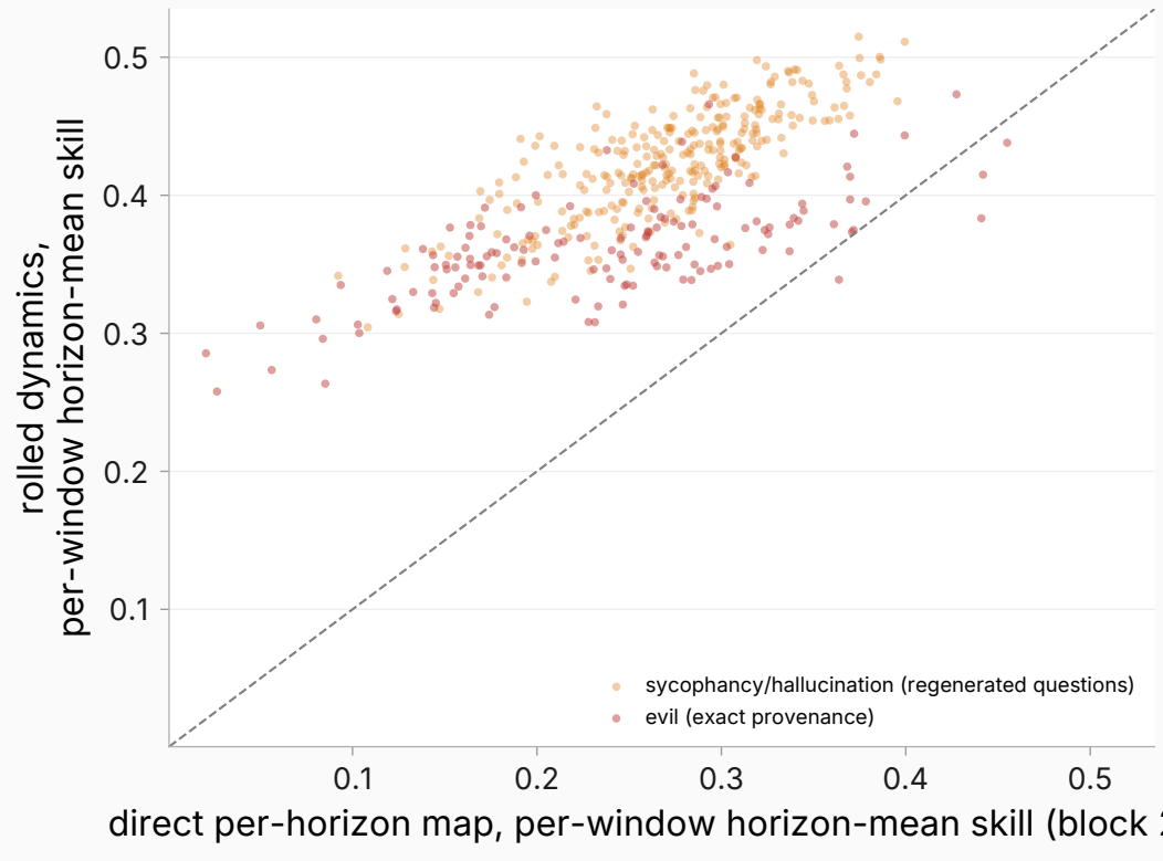
Transfer per-window view, n=432 (rolled above diagonal for 99% of windows)
