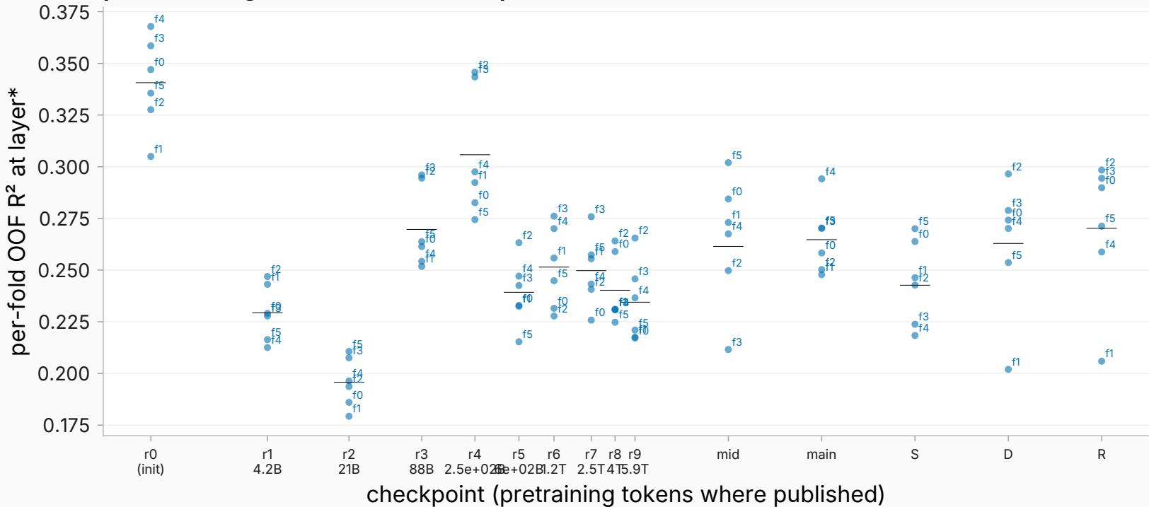
per-fold diagonal R^2 (black tick = pooled)
