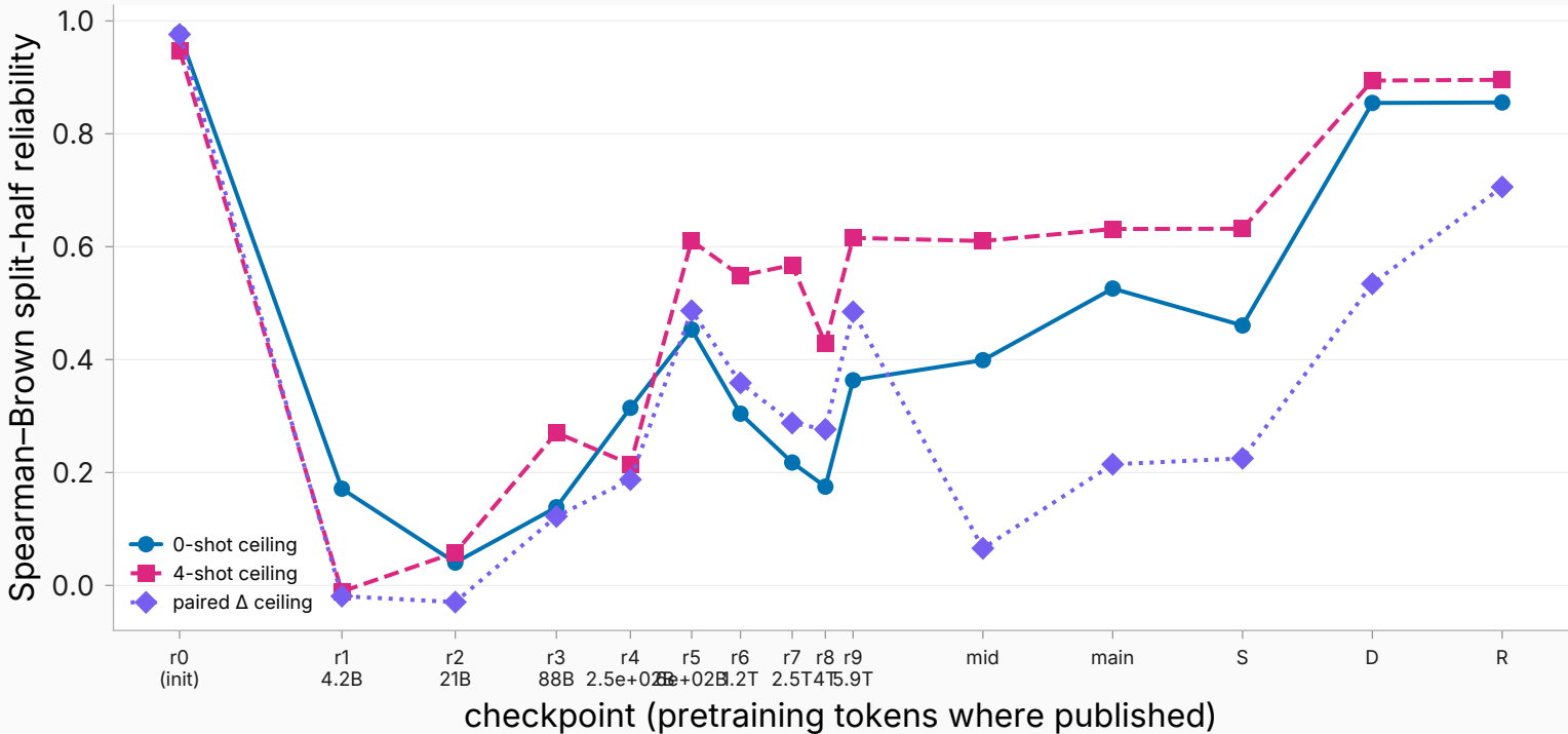
repeat-generation ceilings per rung
