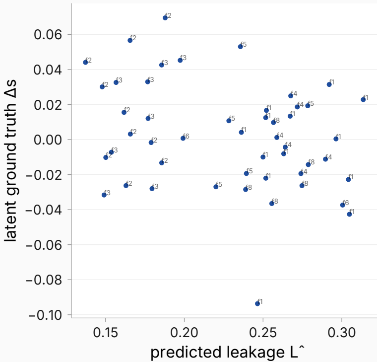
mk_librarian_posonly_d1_seed42 ( \rho = -0.239 )
