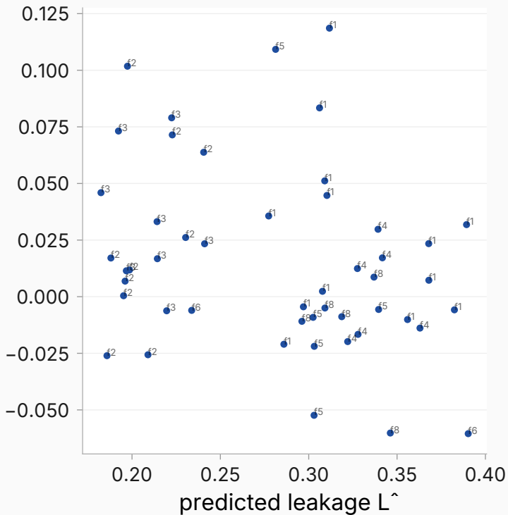
mk_programmer_posonly_d1_seed42 ( \rho = -0.242 )
