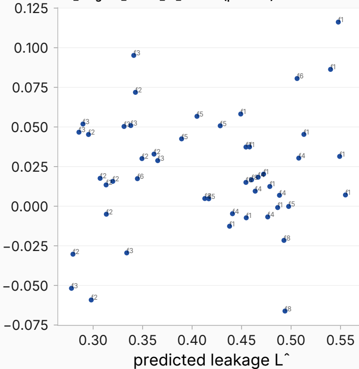
mk_surgeon_contra_d1_seed42 ( \rho=0.041 )
