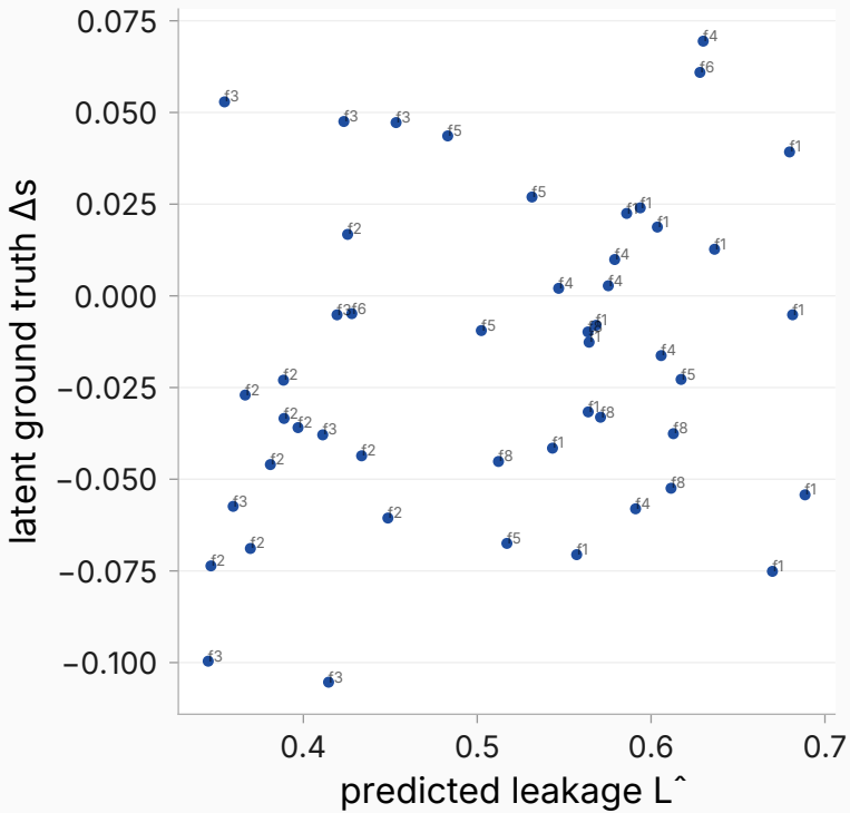
mk_surgeon_contra_d2_seed42 ( p=0.274 )
