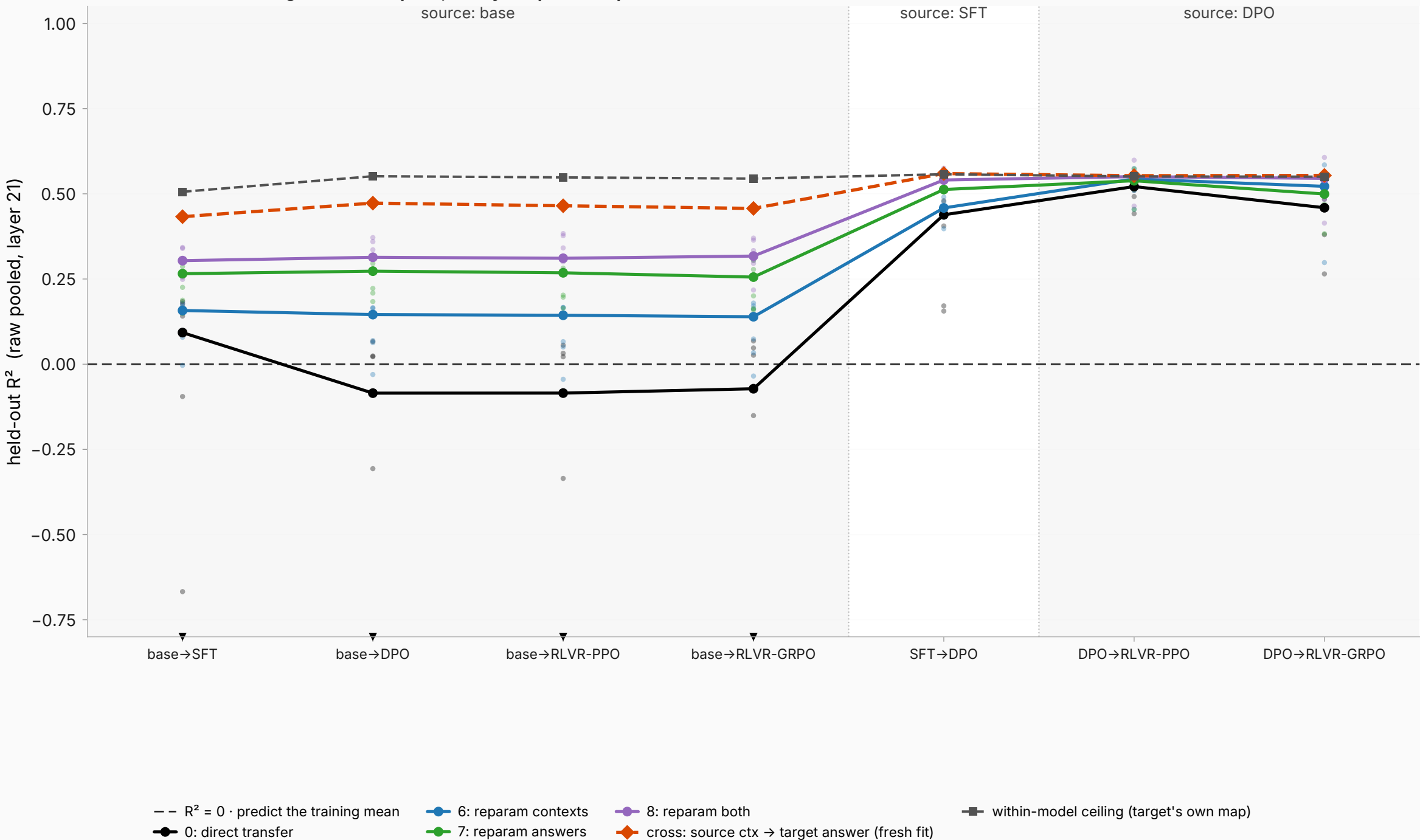
Every forward pair of the Tülu-3 ladder: how much of the context→answer map survives median over 7 non-degenerate corpora, every corpus overplotted
