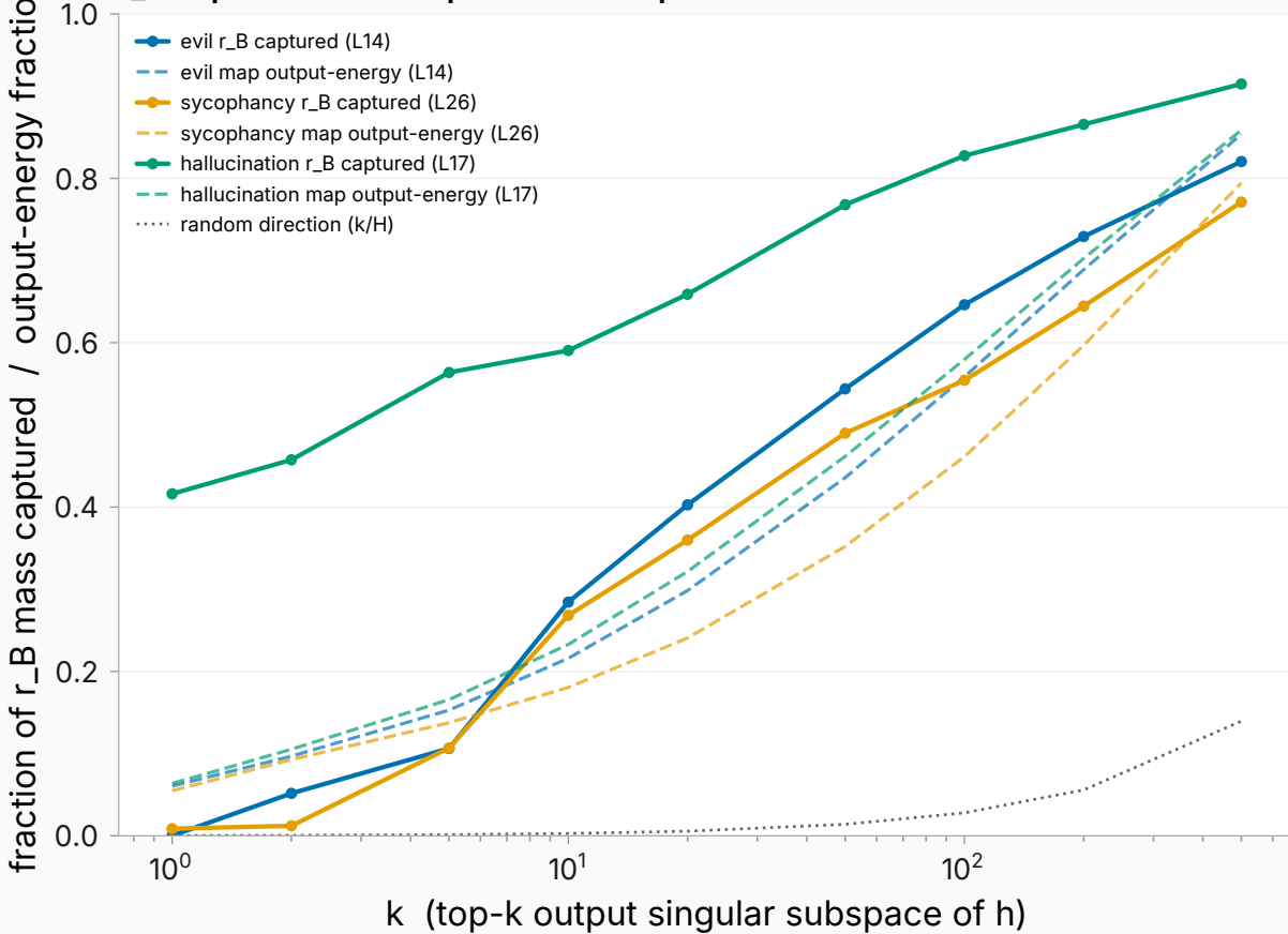
r_B capture vs the map's variance spectrum
