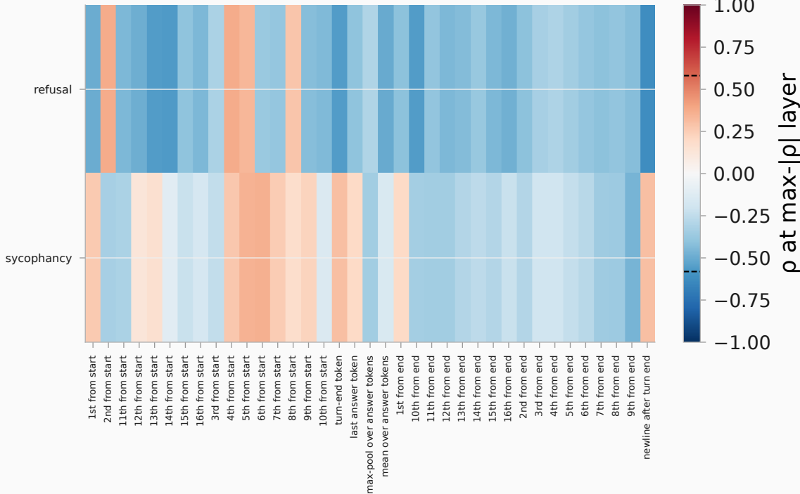
fixed behavior-direction read-out null band (97.5th pct of max): |\rho| \leq 0.581
