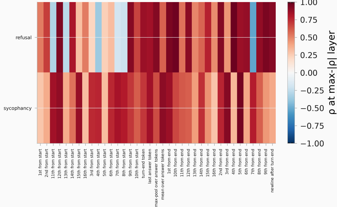
trained leave-one-out ridge read-out null band (97.5th pct of max): |\rho| \leq 0.993
