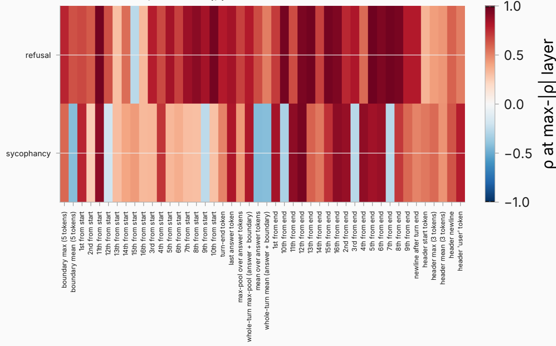
trained leave-one-out ridge read-out null band (97.5th pct of max): |\rho| \leq 0.994
