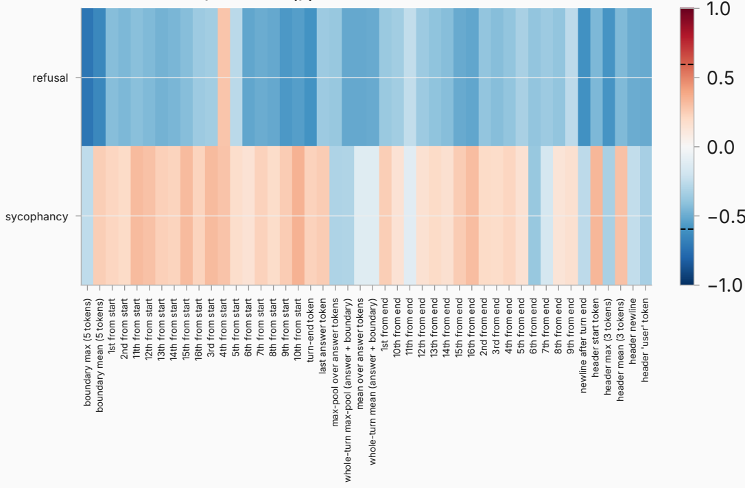
fixed behavior-direction read-out null band (97.5th pct of max): |\rho| \leq 0.595
