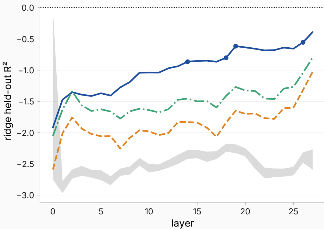
Pretrained · naturalistic (n = 1738)
