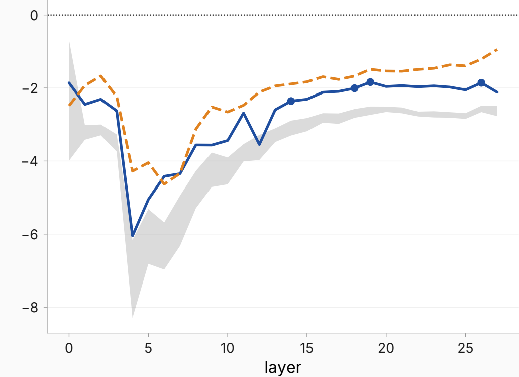
Pretrained · chat (n = 1999)
