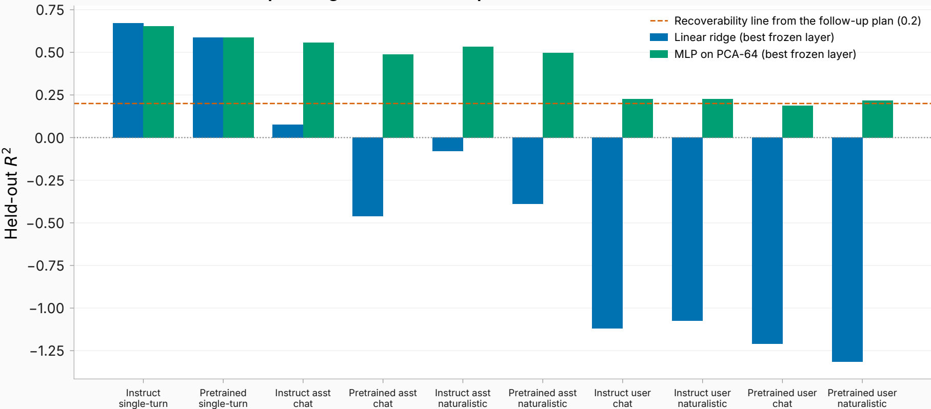
Linear vs nonlinear map strength — all 10 MLP-probed cells (both rounds)
