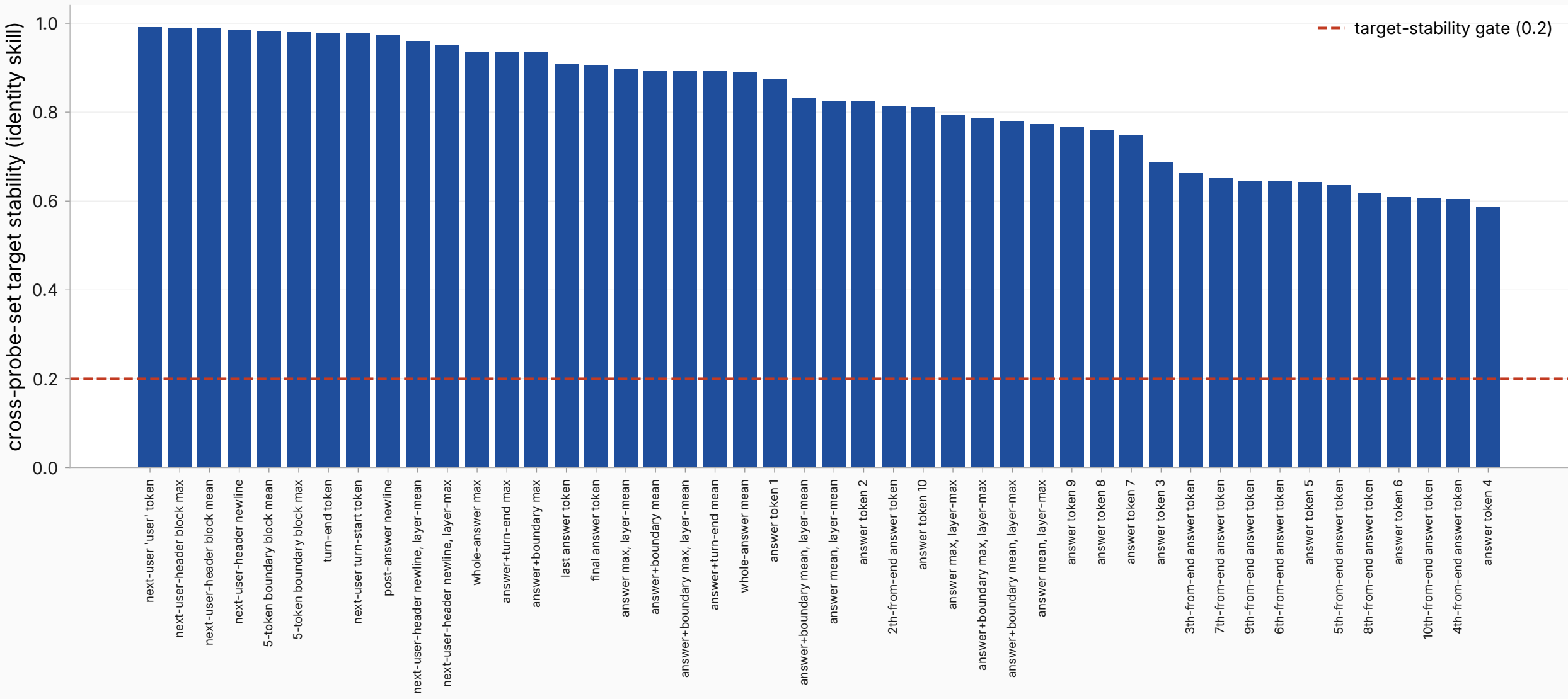
Target-stability ceiling per answer family (pool-A targets predicting pool-B)
