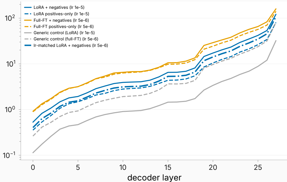
sycophancy mean-shift norm — response arm
