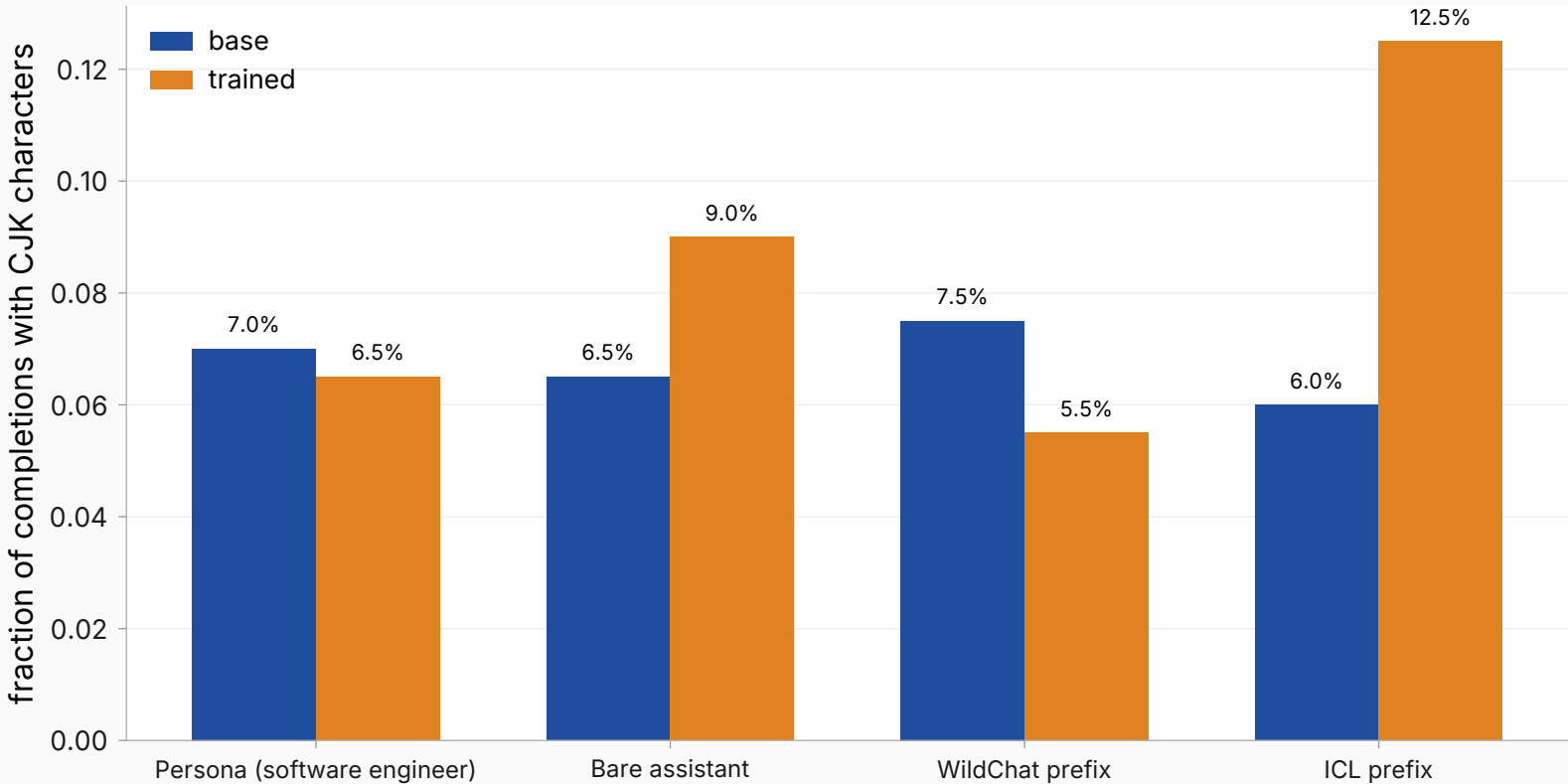
Language-intrusion audit on the Tier-2 verdict pools (n=200 per arm)
