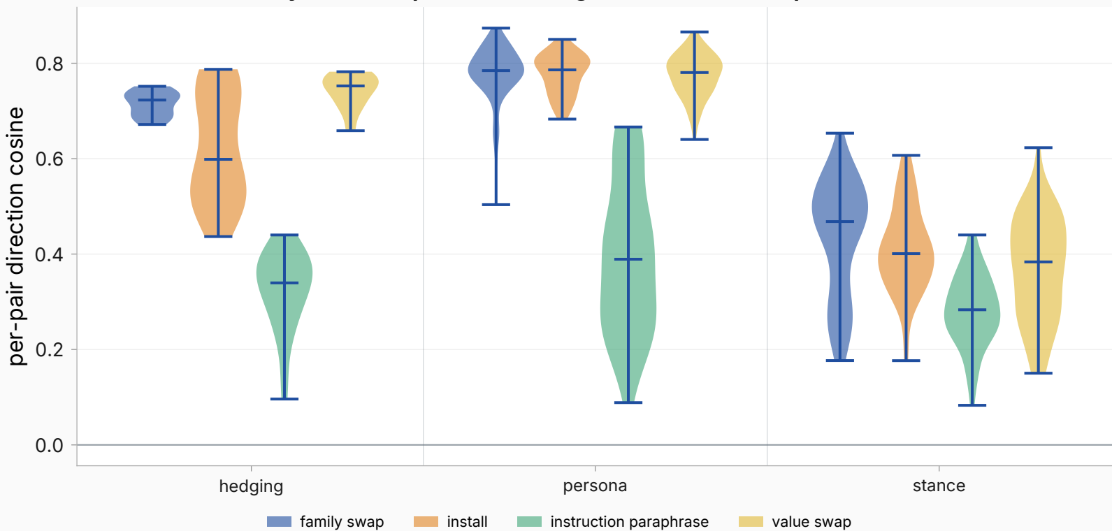
Direction cosine by axis and pair class (single-turn frozen map)
