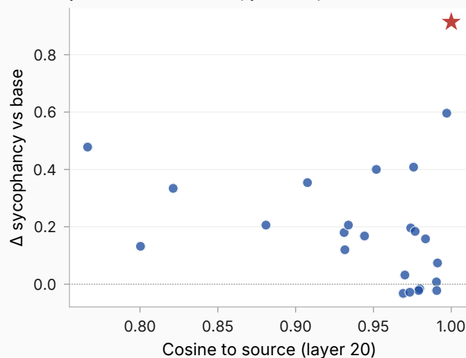
Software engineer ✓ \rho=-0.34 (#99: -0.20), p=0.104 , n=23
