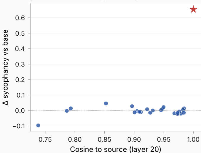
Qwen default × \rho=-0.17 (#99: -0.69), p=0.428 , n=23
