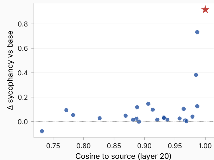
Generic assistant × \rho=+0.27 (#99: -0.44), p=0.202 , n=23
