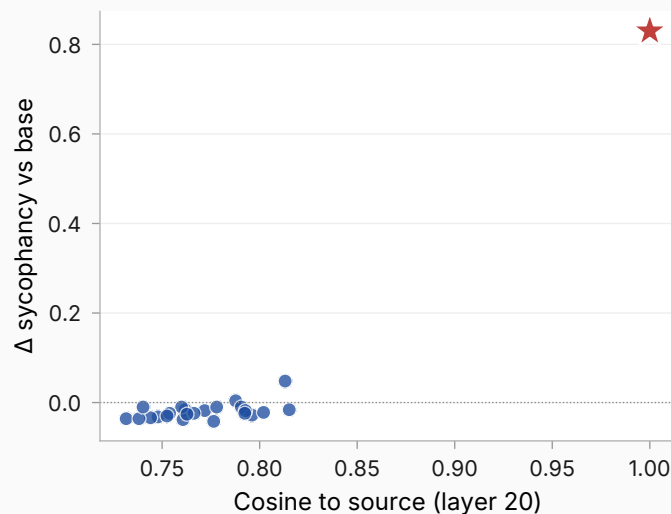
Comedian ✓ \rho=+0.44 (#99: +0.43), p=0.035 , n=23
