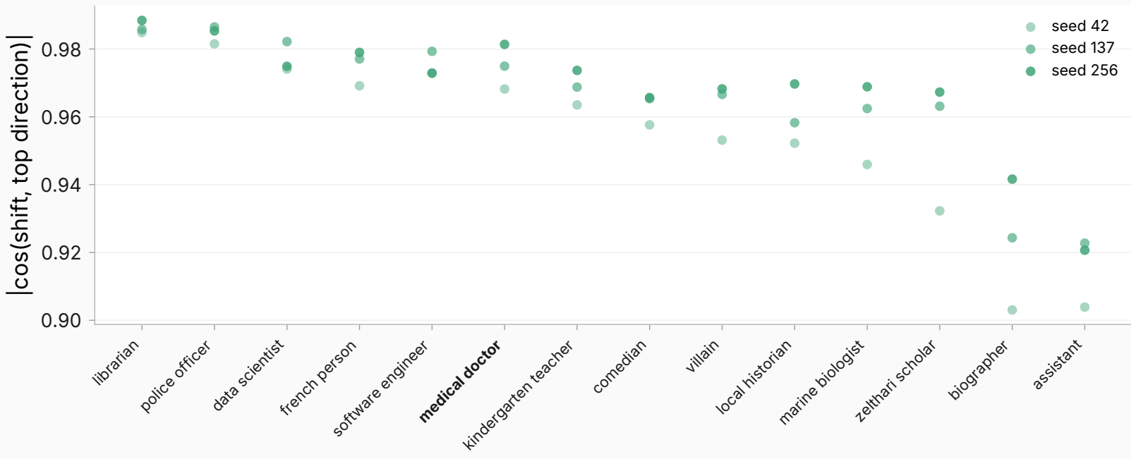
Benign SFT arm: per-persona alignment, sorted by 3-seed mean (bold = source-domain persona)
