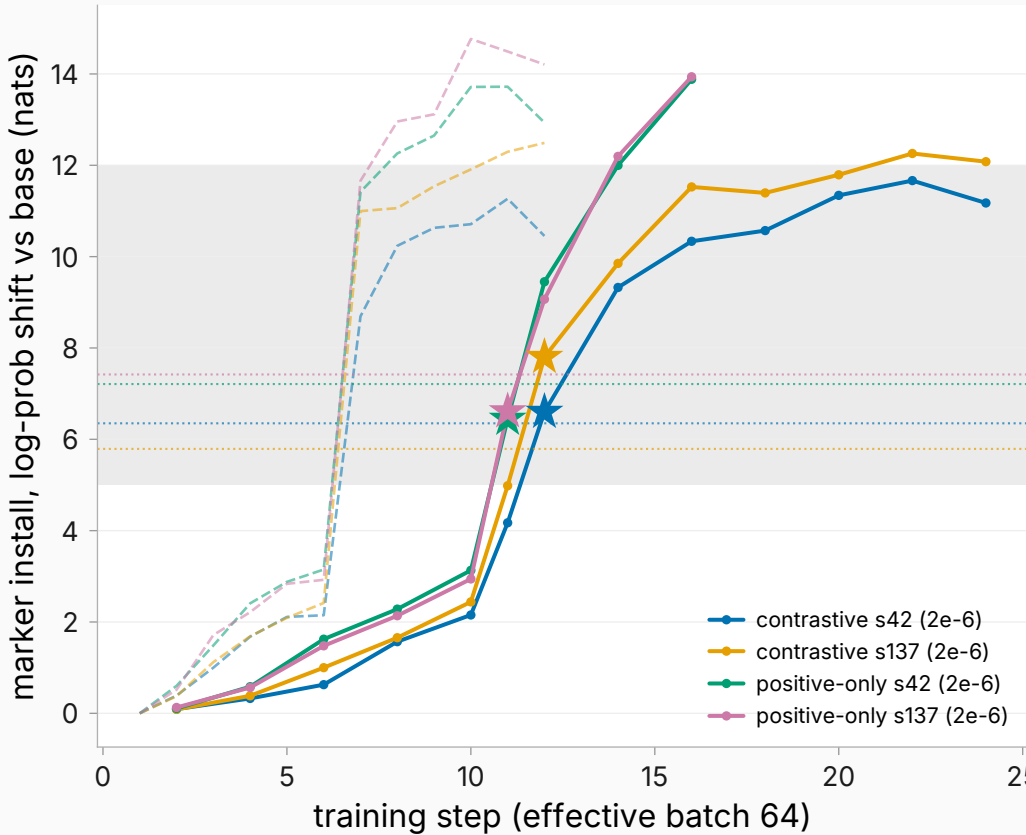
Marker full fine-tune install per step: learning rate 2e-6 (solid, this round) vs 5e-6 (dashed, executed run); stars = selected rungs
