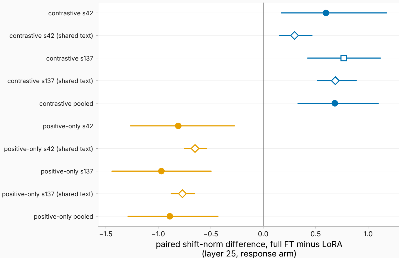
Marker method contrast at matched install (learning rate 2e-6 full fine-tune)
